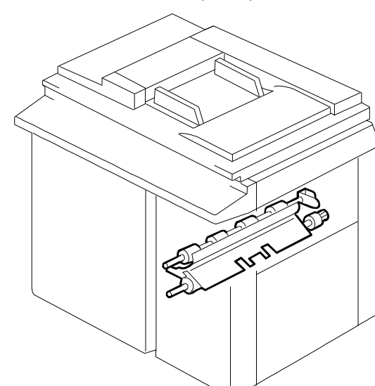
12.2ND FEED ROLLERS (C228)
