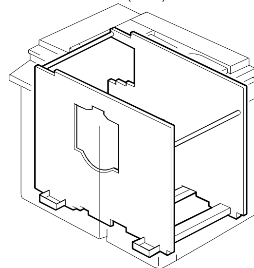
3.FRAME SECTION 1 (C228)
