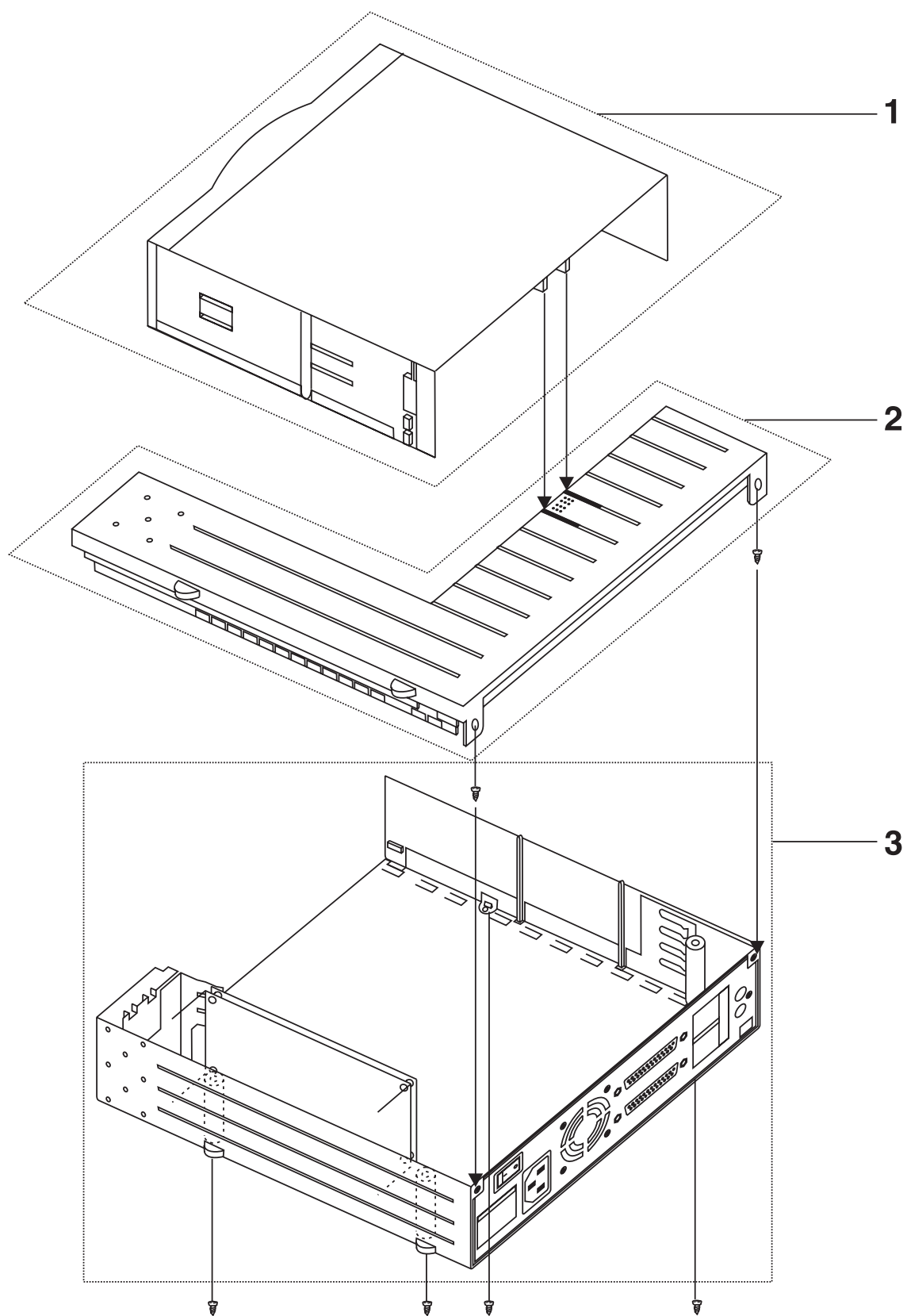
FIGURE 1. EXTERNAL PARTS
