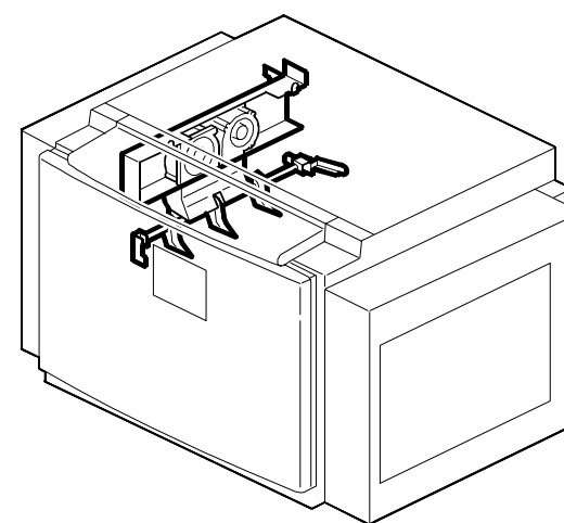
12. Paper Exit Section 1 (C639)
