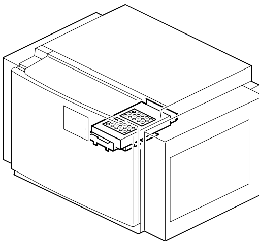
11. Paper Transport 2 (C639)
