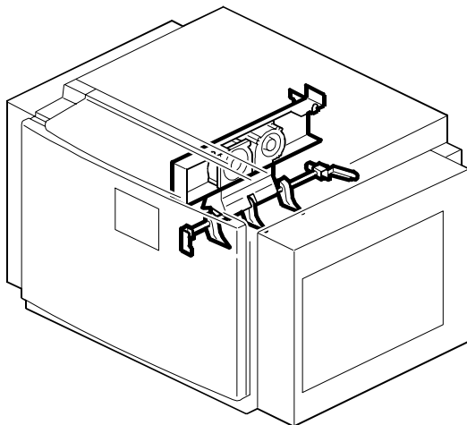
10. Paper Transport 1 (C639)
