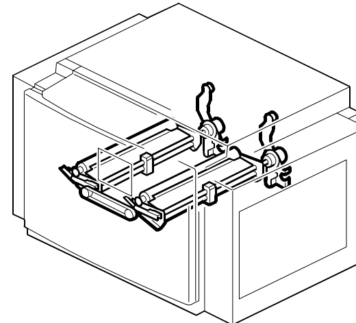
9. Pressure Roller Section 1 (C639)
