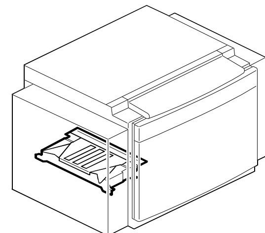
12. Paper Exit Section 2 (C593)
