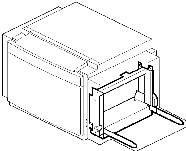
4. Paper Feed Section 2 (C593)
