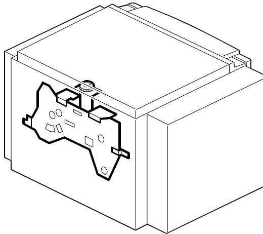
14. Drive Section 1 (C593)
