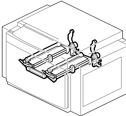
8. Pressure Roller Section 1 (C593)
