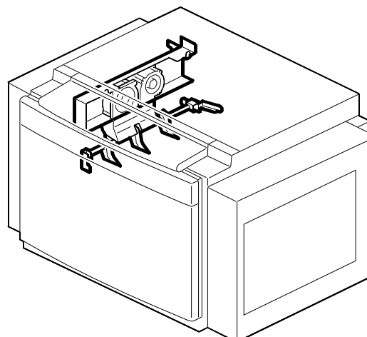
11. Paper Exit Section 1 (C593)
