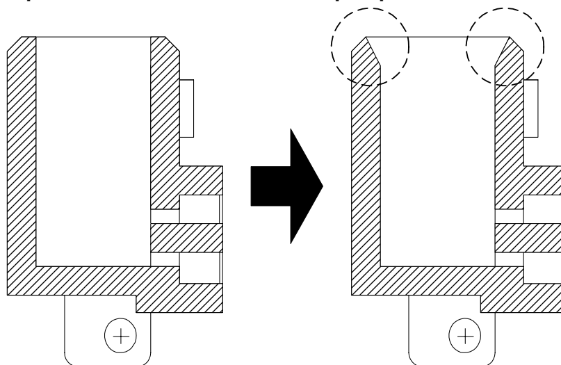
A partial cross section of the ink pump case
