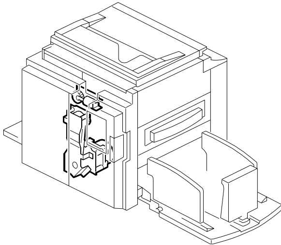
19. Drive Section 1 (C238)
