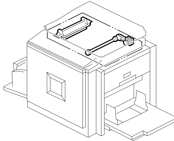
5. Scanner Unit 3 (C264)
