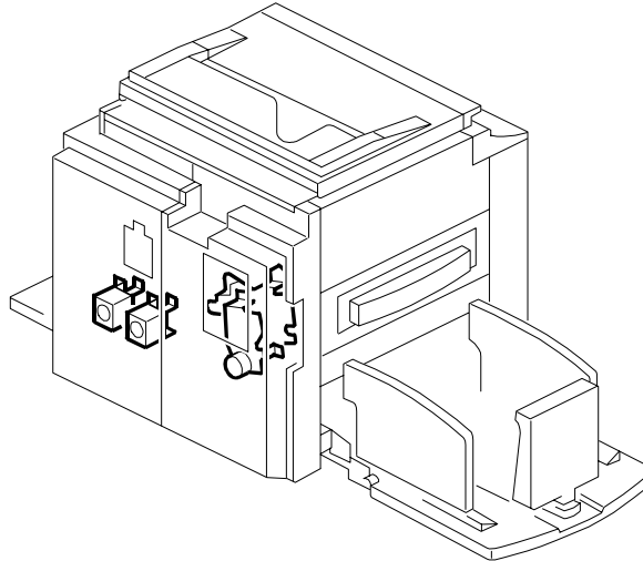
23. Drive Section 2 (C264)
