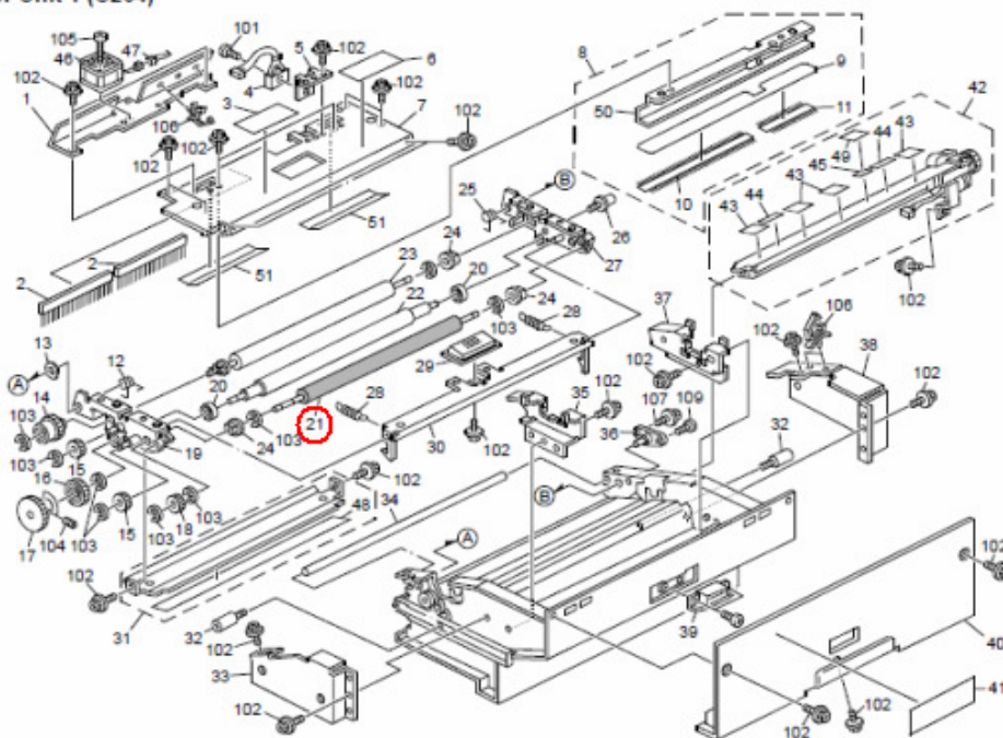
9. Plotter Unit 1 (C264)
