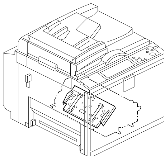
17. Duplex Unit 1 (C269)
