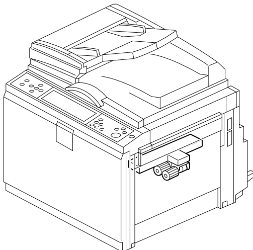
10. Paper Feed Section 3 (C269)
