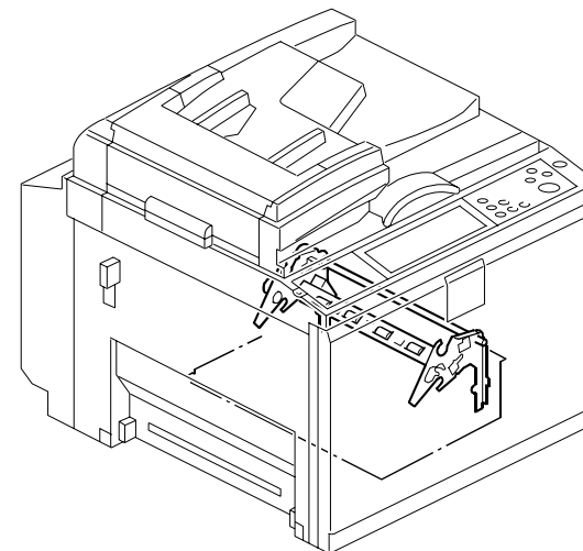
21. Duplex Unit 5 (C269)
