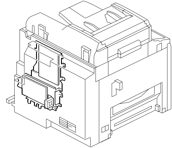
51. Electrical Section 1 (C269)
