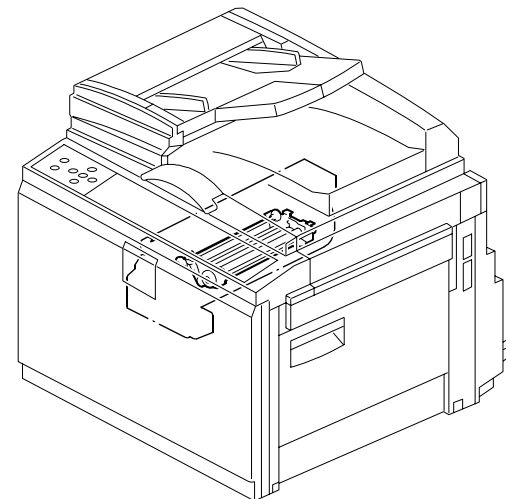
30. Drum Unit 5 (C269)
