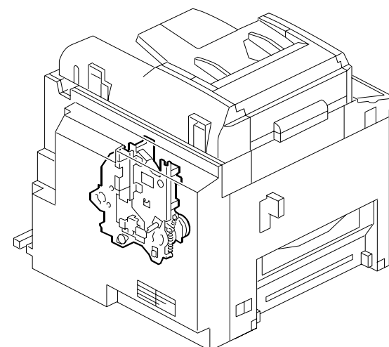
6. Drive Section 3 (C269)
