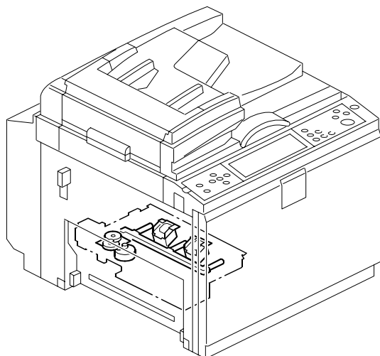
16. Paper Delivery Unit 3(C269)
