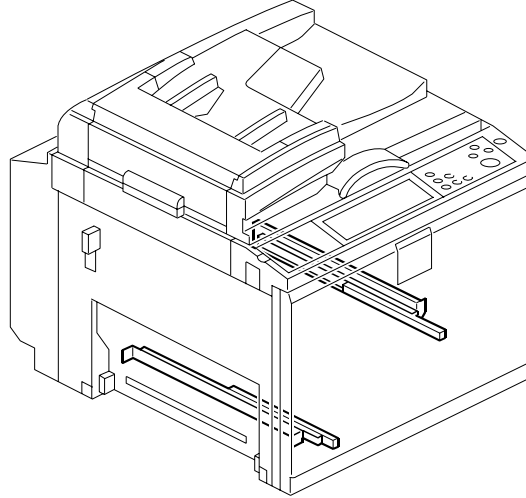
50. Frame Section 6 (C269)
