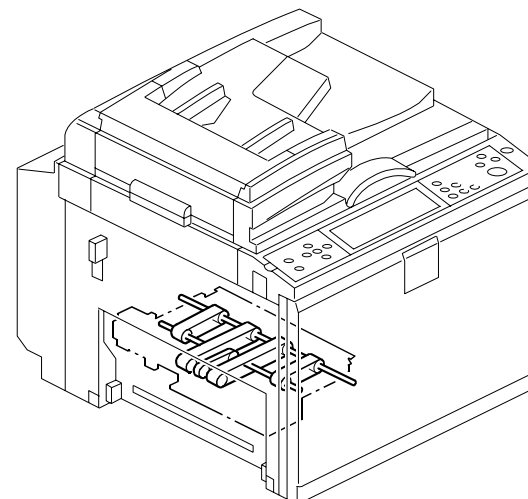
15. Paper Delivery Unit 2(C269)
