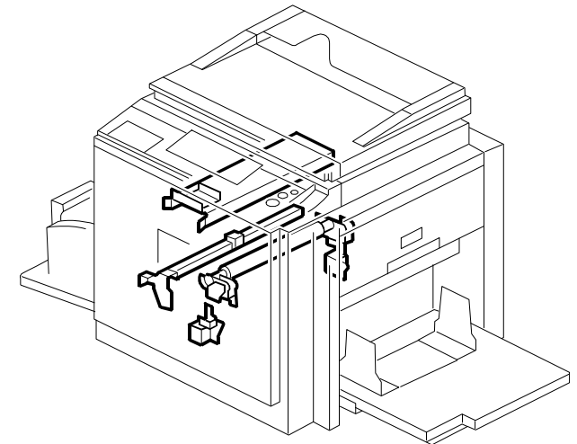
12. Press Roller Section (C272/C273)
