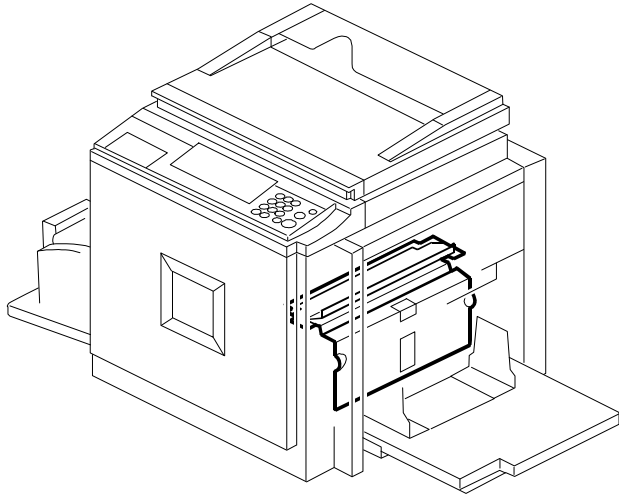
7. Paper Feed Section (C272/C273)
