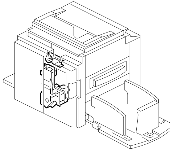
23. Drive Section 1 (C272/C273)
