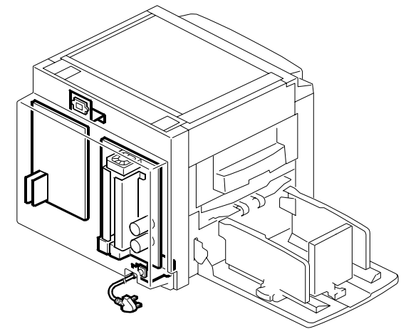
21. ELECTRICAL SECTION 1 (C267)
