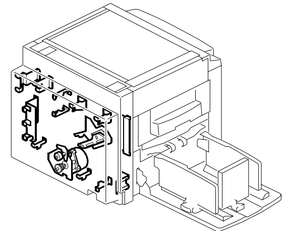
24. DRIVE SECTION 2 (C267)
