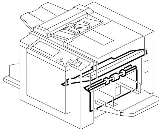
5. Paper Registration (C274)
