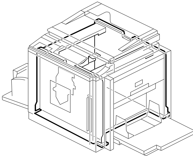
28. Frame Section (C277/C278/C279)
