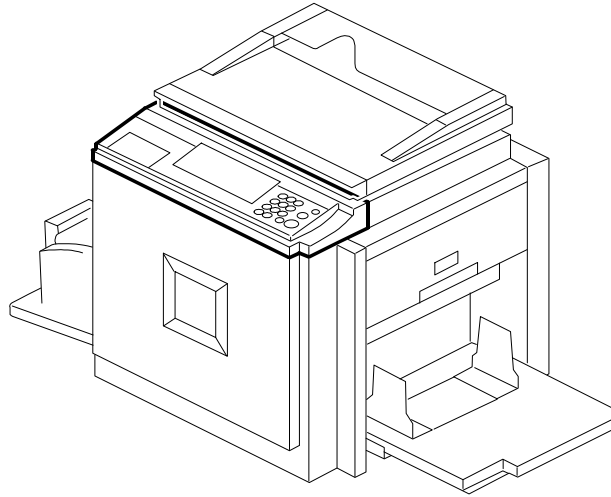
2. Operation Panel (C277/C278/C279)
