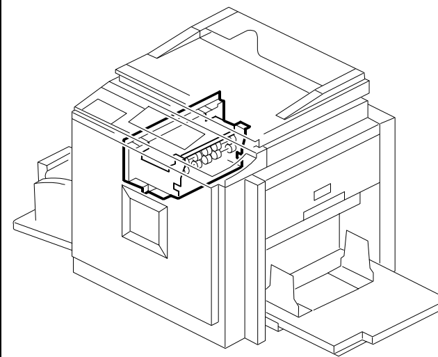
21. Master Eject Unit 1 (C277/C278/C279)
