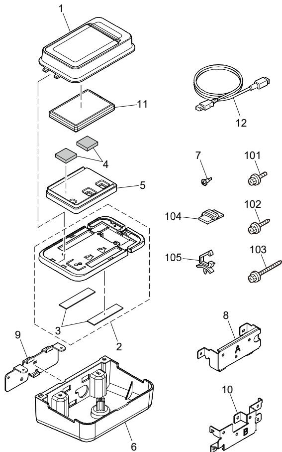
NFC Card Reader Type P11
