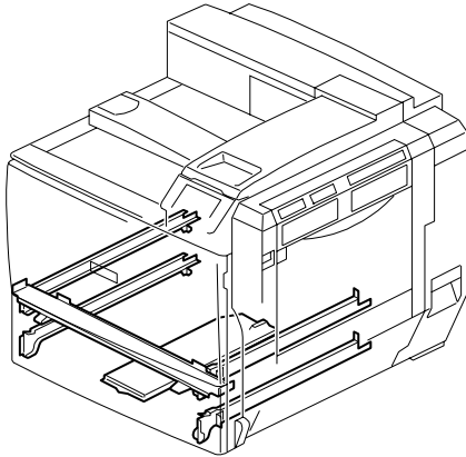
34. Frame Section (M132)
