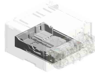
U003 PAPER CASSETTE
