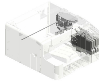
U007 CARRIAGE UNIT/INK SUPPLY UNIT:(for J017/J019)
