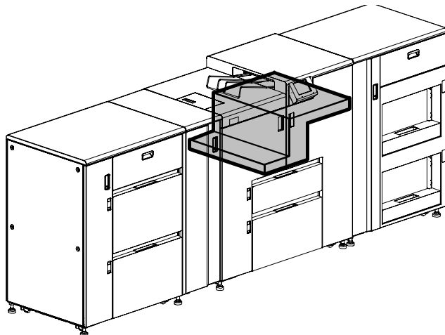
16. Paper Feed Module 3 (G155)
