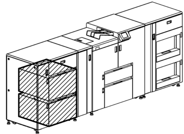
51. Feeder Hopper Ass'y 2 (G155)
