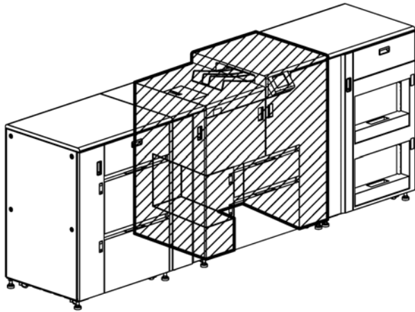
1. Final Ass'y 1 (G155)
