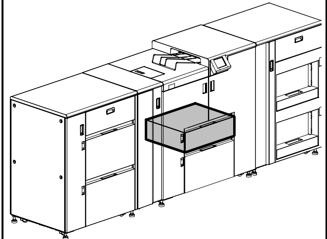
12. Small Hopper Ass'y 1 (G155)
