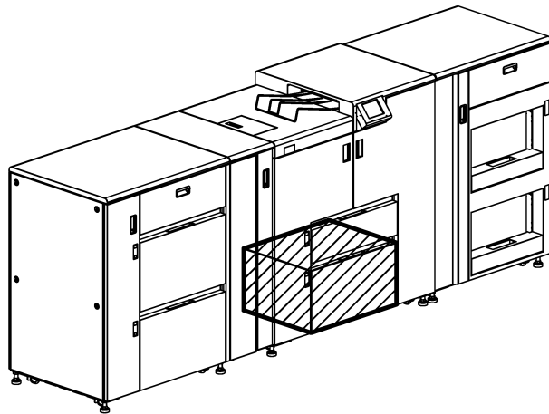
10. Large Hopper Ass'y 1 (G155)
