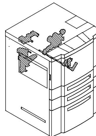
9. Paper Feed Drive (G150)
