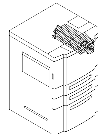
6. Development Unit (G150)
