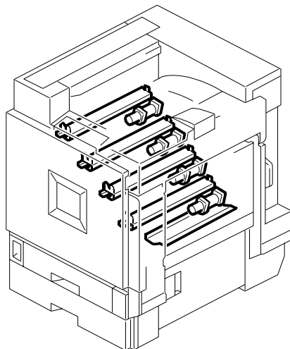
26. Waste Toner Transfer Section (G080)
