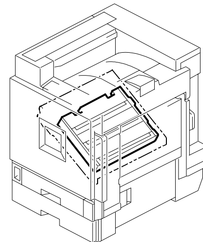
18. Transfer Unit 4 (G080)
