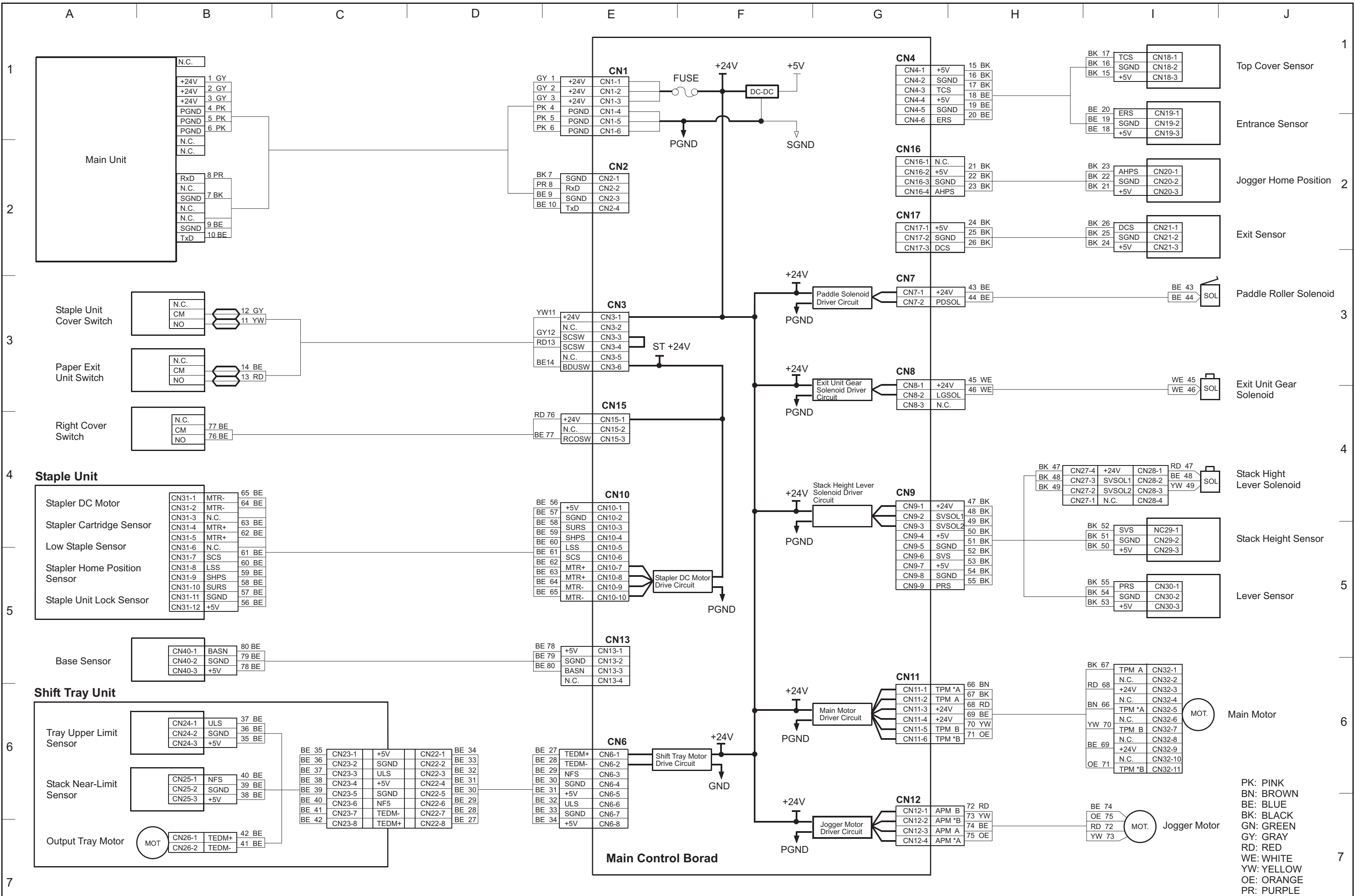
POINT TO POINT CIRCUIT DIAGRAM (500-SHEET FINISHER: G314)
