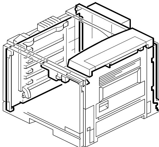
2. EXTERIOR 2 (G071)
