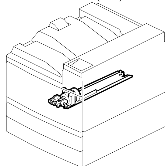
9.TONER HOPPER UNIT (G035)
