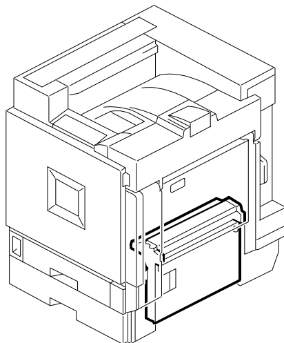
8. Vertical Transport Section (G060)
