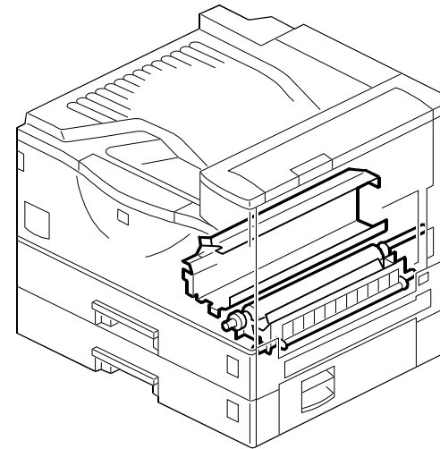
9. PAPER REGISTRATION (G062)
