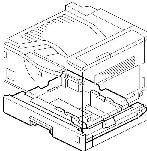
11. PAPER TRAY 2 (G062)
