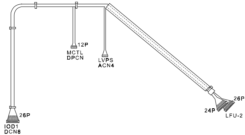
2 Harness WH (B)
