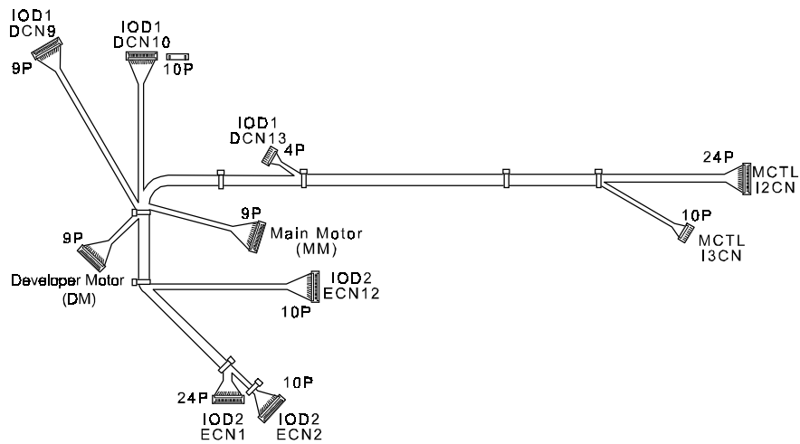
2 Harness WH (B)
