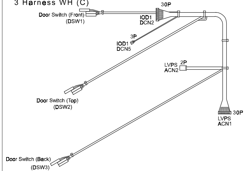
3 Harness WH (C)
