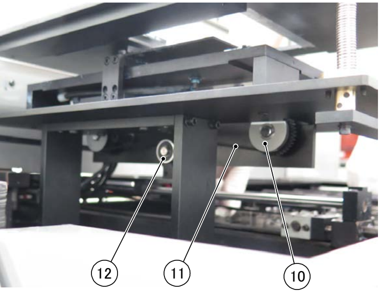
VIEW "B"
