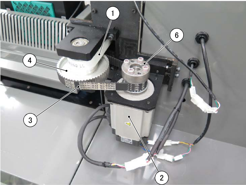
VIEW "C"
