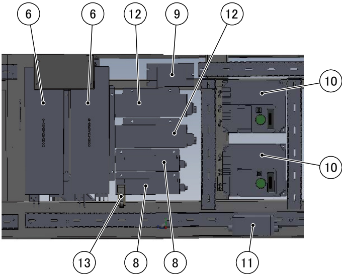
VIEW "C"
