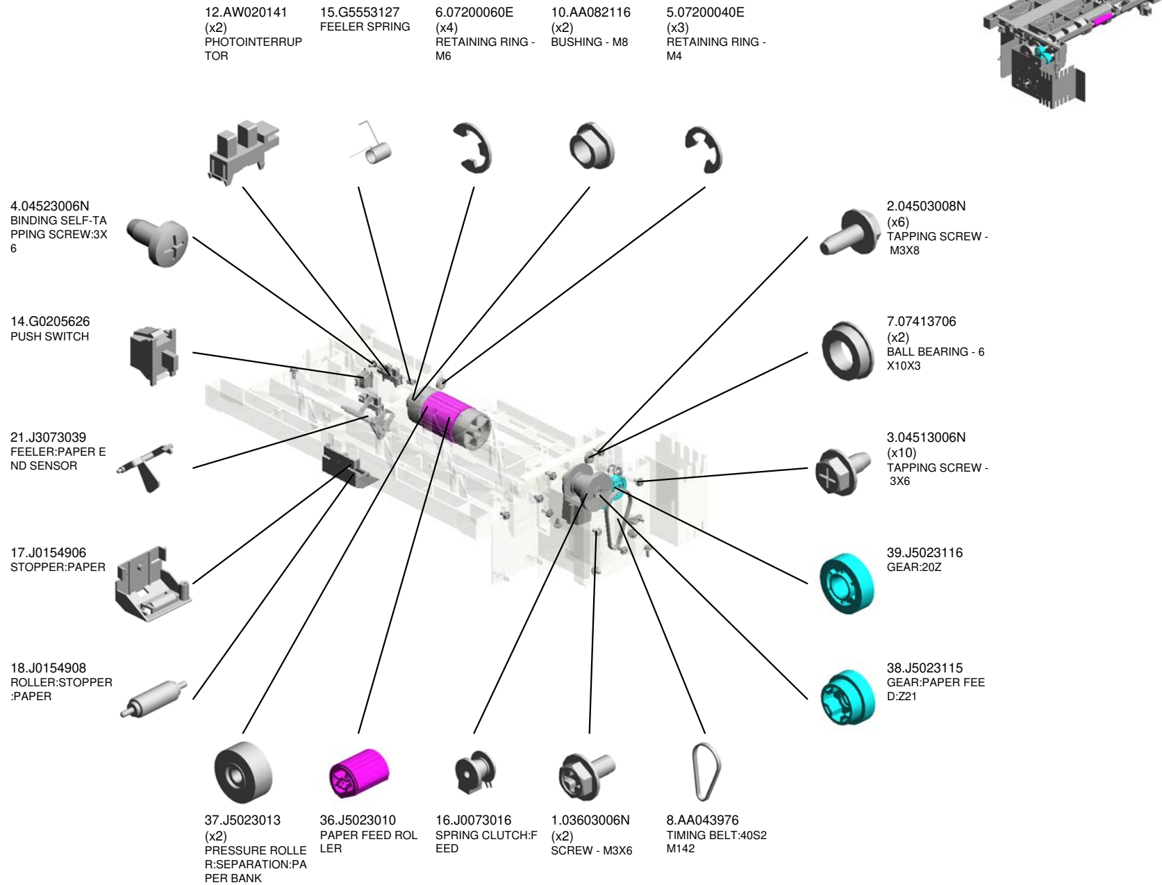
19.J3073500 PAPER FEED UNIT :MUSTARD-C
