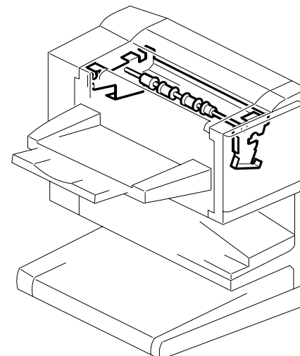
6. PAPER TRANSFER 3 (B602)
