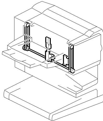
16. PAPER TRAY DRIVE (B602)
