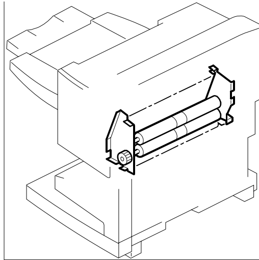
14. PAPER FOLDER 4 (B602)
