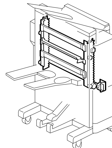
15. TRAY DRIVE SECTION (B546)
