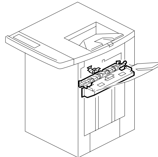
15. PAPER EXIT SECTION 2 (B706)
