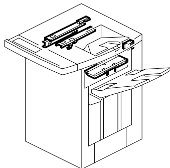
16. Shift Tray Transport 1 (D707)
