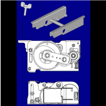
17.B7936400 [A] STAPLER:SERVIC E PARTS:ASS'Y 202001-01 O/O
