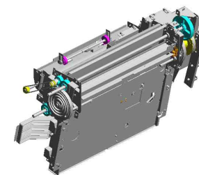
106.D3FQ4801 PAPER CRIMP SUB-UNIT:ASS'Y
