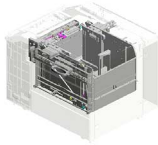
U002 PAPER FEED
