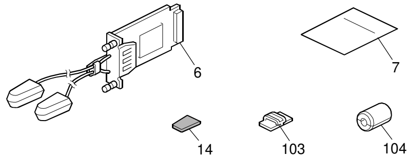
IEEE802.11a/g Interface Unit Type J (D377-01/02)
