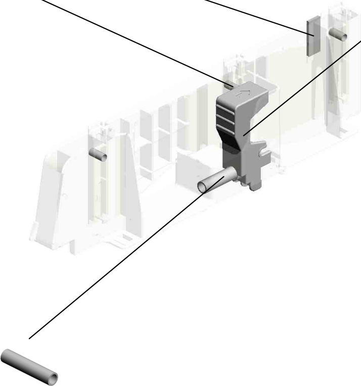
58.D1492827 COMPRESSION SP RING:SIDE FENCE: POSITIONING
