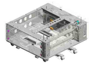
U004 MAIN FRAME
