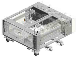
U005 MAIN FRAME
