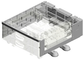
U001 EXTERIOR
