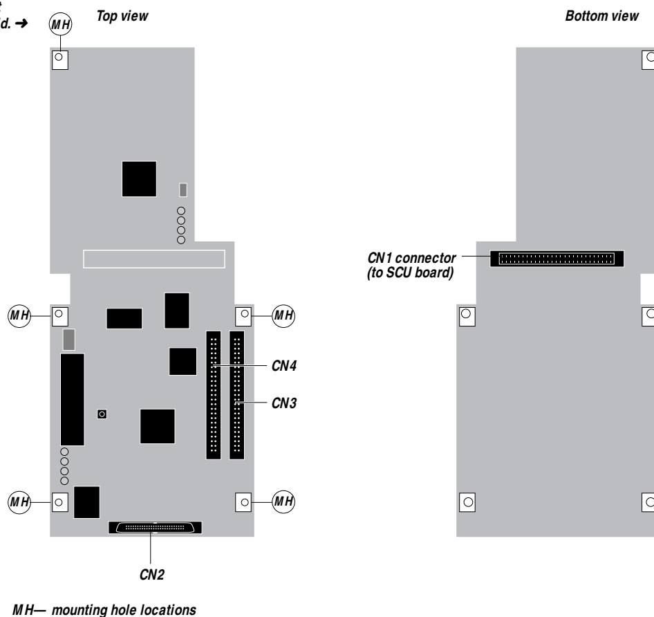
Figure 3-14 EXU board (top and bottom view)
