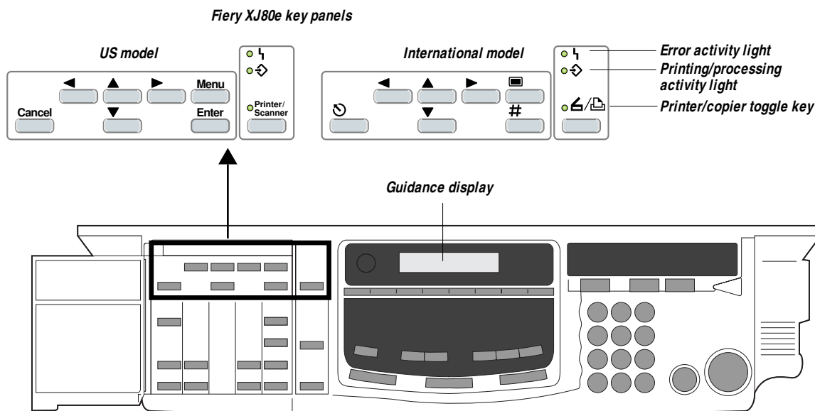
Figure 2-26 Operation Panel
