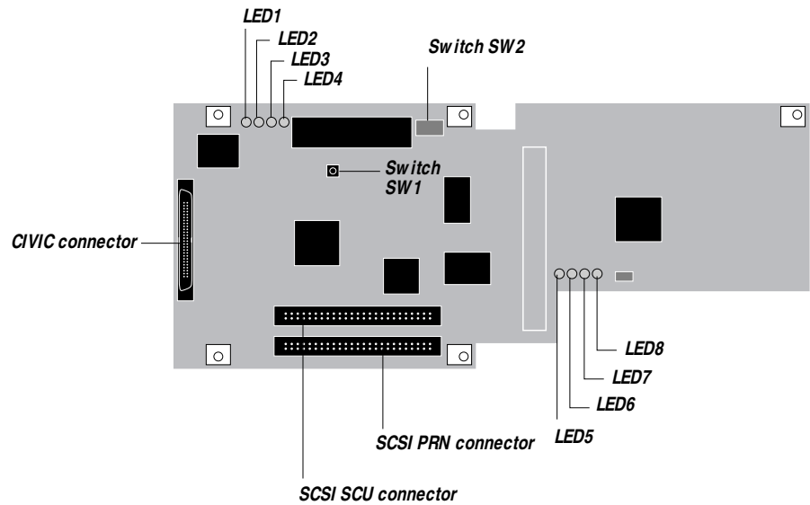
Figure 6-5 EXU board
