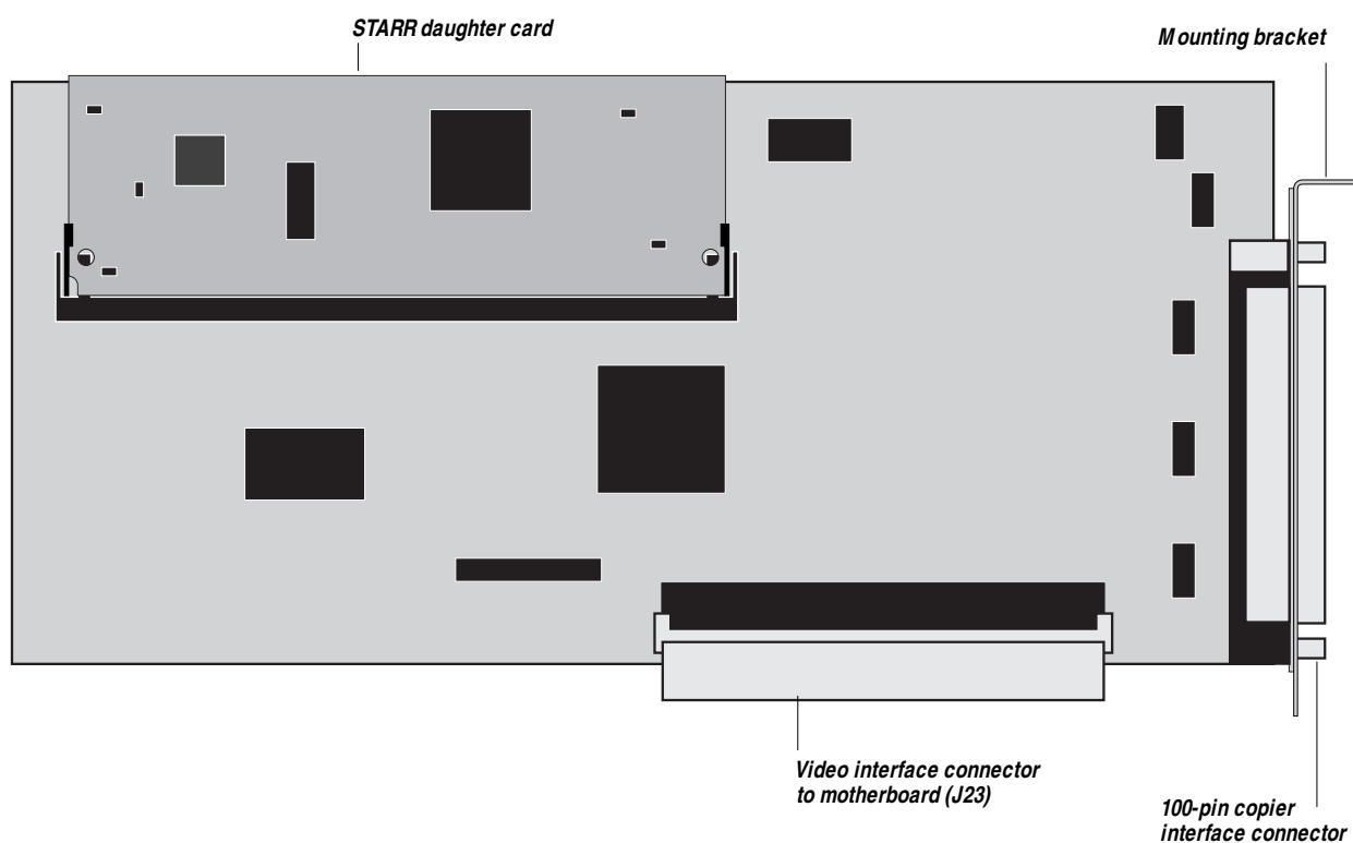
Figure 5-9 Diagram of the Fiery XJ BP100 video interface board
