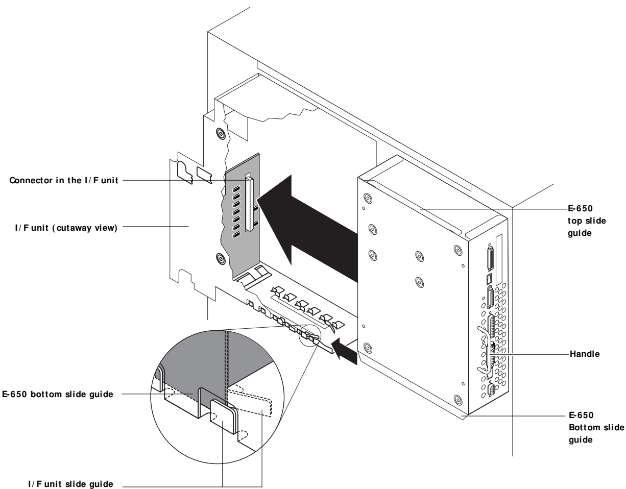
FIGURE 2-4 Installing the E-650 in the I/F unit
