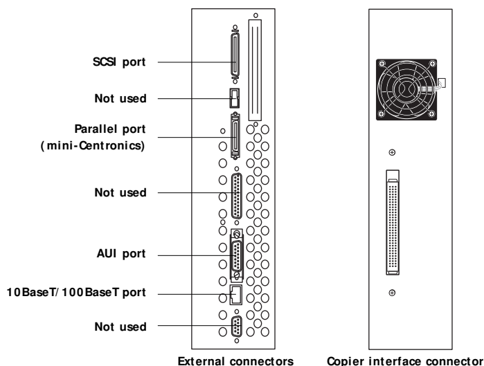
FIGURE 5-2 External connections
