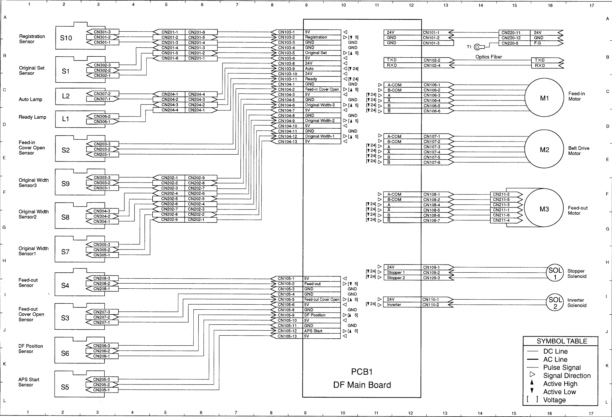
ARDF(A548) POINT TO POINT DIAGRAM
