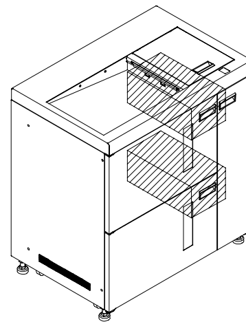
9. Off Set Section (G851/G852/G859/G860)
