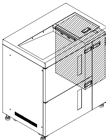
8. Paper Feeder (G851/G852/G859/G860)
