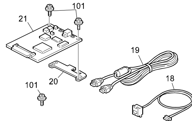
ISDN G4 Interface Unit
