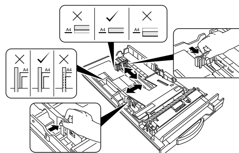
[Main Cassette]
