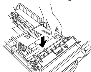
[Main Cassette]
