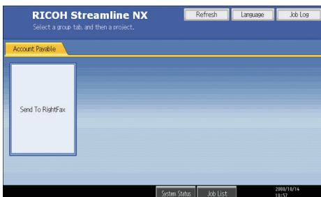
Fig. 4: Group/Project Screen
