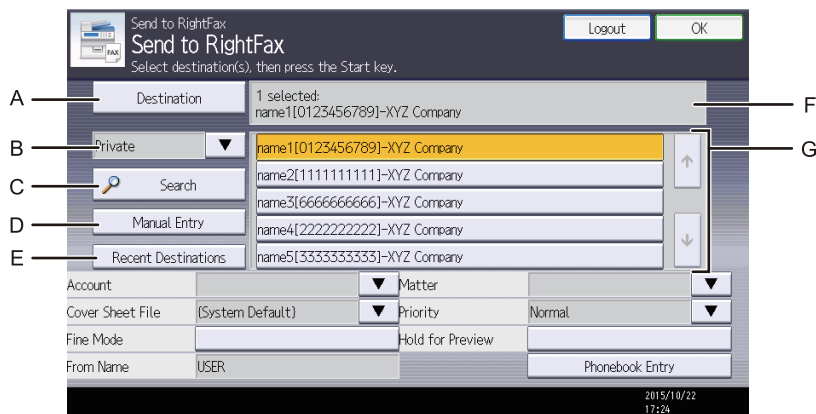
Fig. 6: Destination Selection Screen
