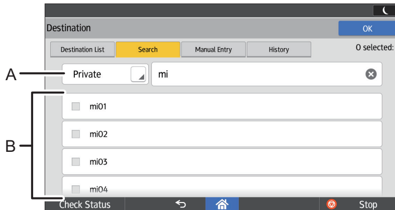
Fig. 17: Search Result Screen
