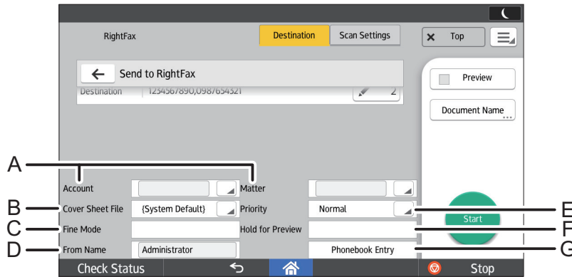
Fig. 18: Destination Selection Screen (2)
