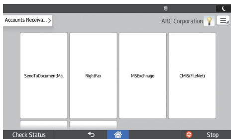
Fig. 13: Group/Project Screen
