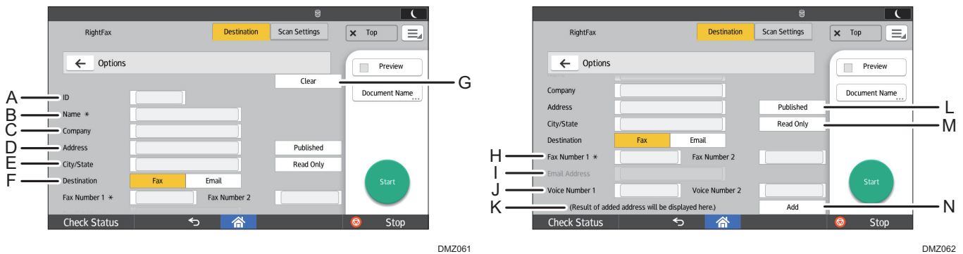
Fig. 19: Options Screen
