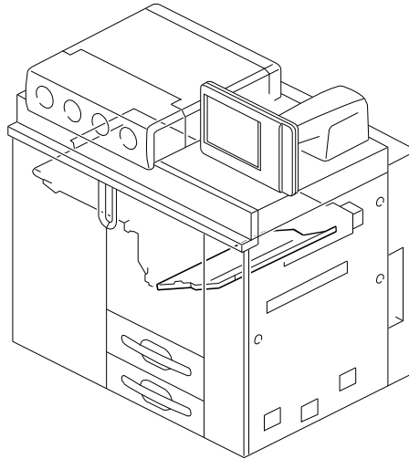
38. Transfer Belt Unit 1 (D095/M077)
