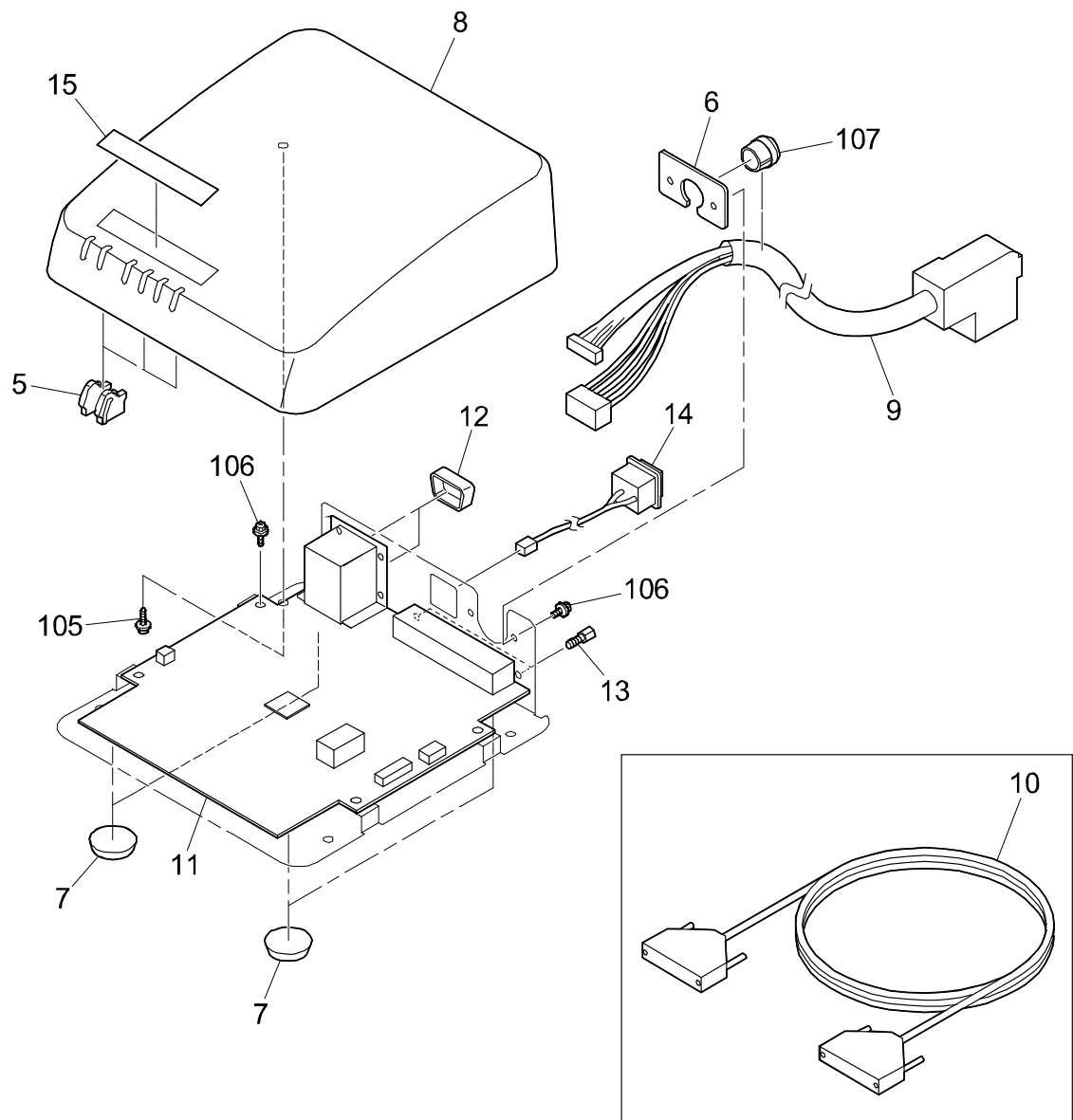
RPIP Interface Box Type S3
