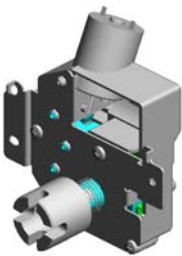
19:04523010N(x 4) BINDING SELF-TAPPING SCREW:3X10
